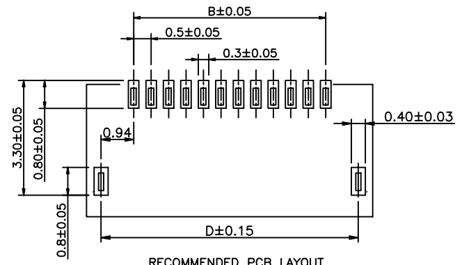
RECOMMENDED PCB LAYOUT TOLERANCE±0.05 (N=CIRCUITS)
