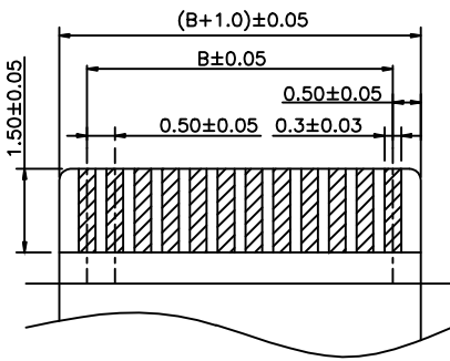
APPLICABLE FPC DIMENSION(REF) (THICKNESS 0.30±0.03)
