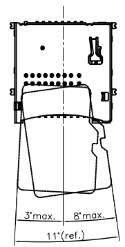
△ Card Insertion Guide Angle
