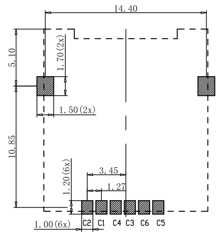
PCB LAYOUT
